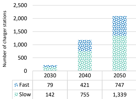
Figure 6.19 – Evolution of charging outlets for the base scenario in the São Miguel Island
