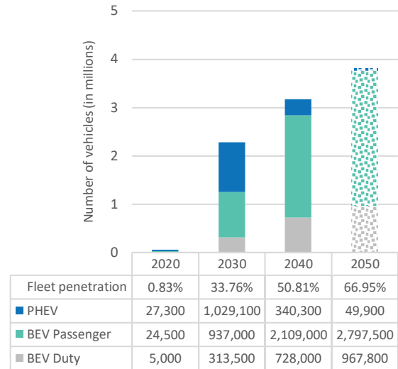
Figure 6.10 – Evolution of light electric vehicles for the progressive scenario
