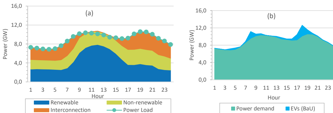
Figure 3.8 – Power generation and demand curve from Greece (a) vs EV charging without management (b), Scenario 2050
