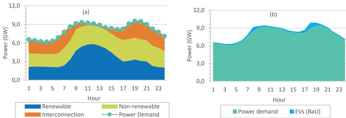
Figure 3.7 – Power generation and demand curve from Greece (a) vs EV charging without management (b), Scenario 2030
